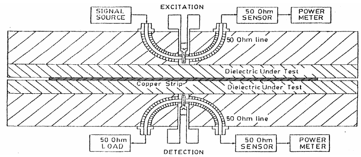
Figure 2: Side view of the fixture design used for Bereskin measurements. A copper strip conductor is sandwiched between two laminate samples, to which a microwave signal is incident through the z-axis of the structure, creating a cavity resonator.
